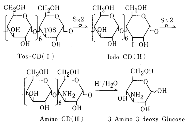
Scheme 1. Suggested Reaction Mechanism for the Synthesis of Regiospecific Amino- \beta -CD (III) from Tos- \beta -CD (I) via Iodo- \beta -CD (II) Intermediate
